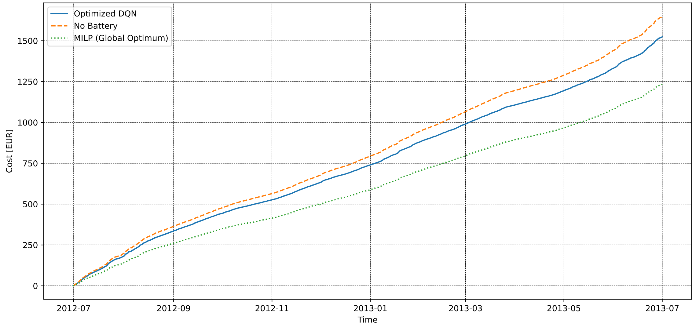
User 65 - Basic Training - Electricity Cost [DQN vs MILP]
